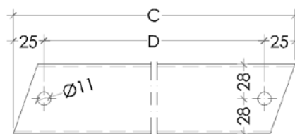
Tracé diagonal
