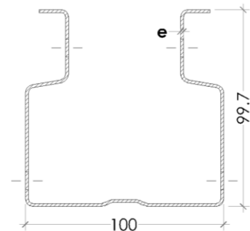
Plan view Upright 100 100
