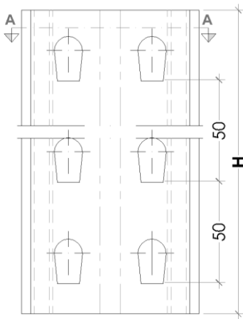
Plan view Upright 80 63
