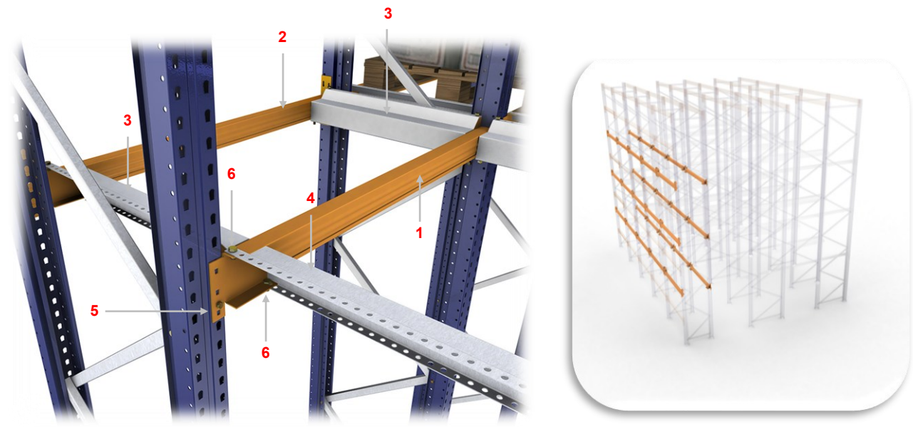
Single/double corbel beams and position in the overall structure
