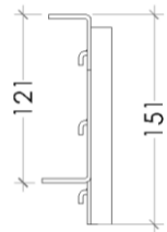
Cross-section 80 corbel
