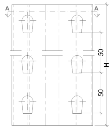
Plan view Upright 100 100
