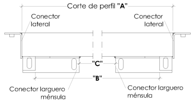
Plan view Single corbel beam
