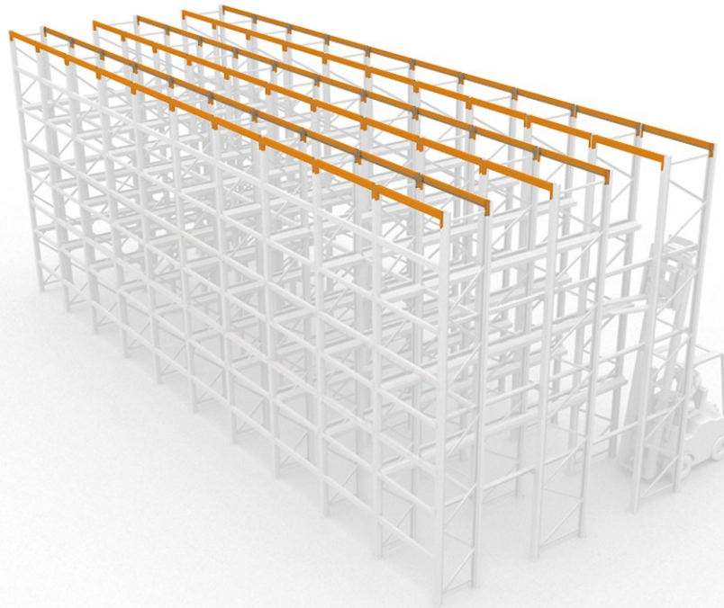
Top beams. Position on top of the structure
