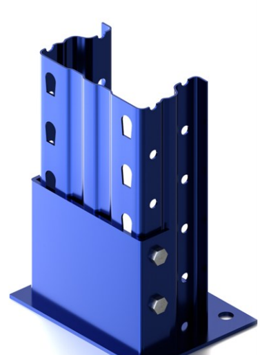
Upright 100 100 with base plate
