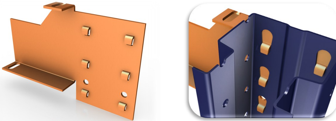
Corbel/upright connections. Close-up of the hooks and position on the upright
