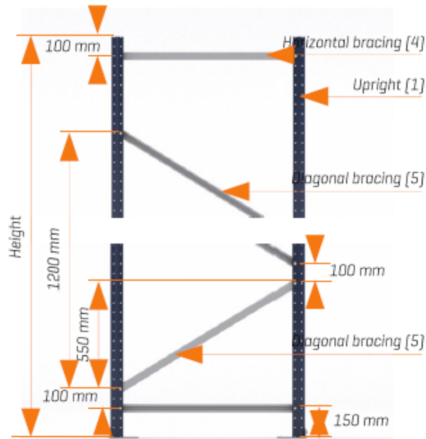
Type 1 assembly scheme
