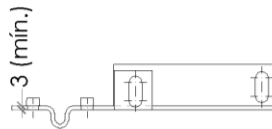
Plan view of 80 left corbel
