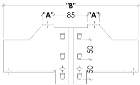
Elevation view of 80 double corbel
