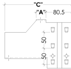
Elevation view of 80 right corbel
