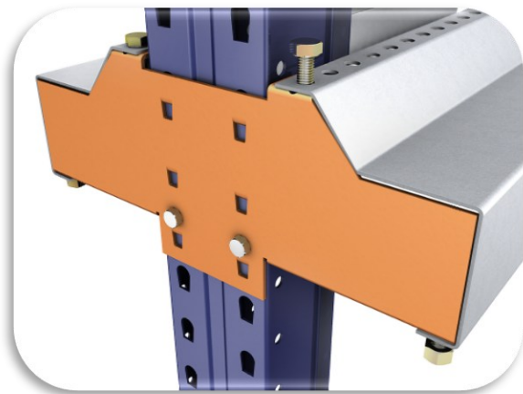
Connection between centring rails and corbels M10x20 bolts
