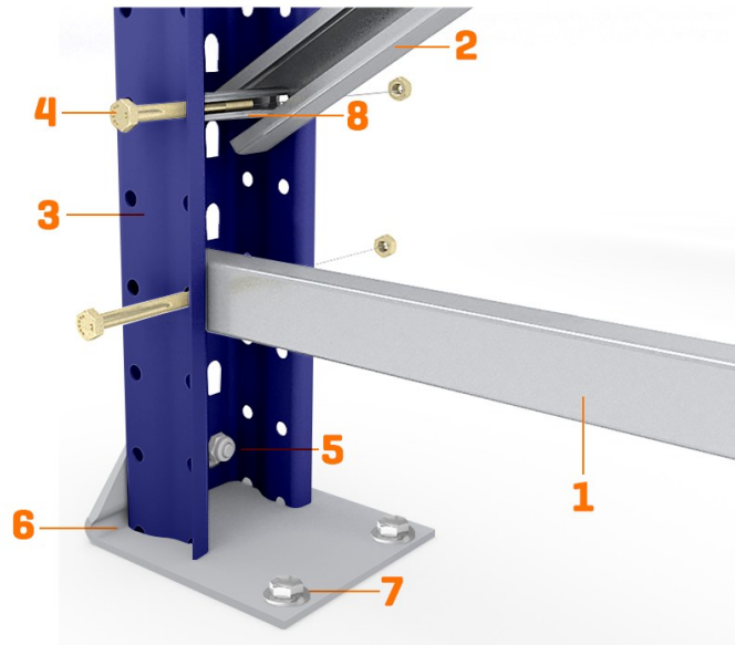
Detailed diagram of bracing elements
