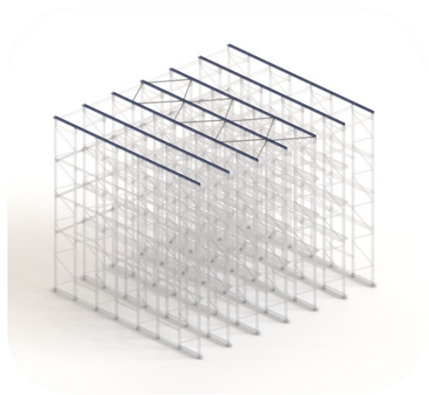
Generic position of bracings
