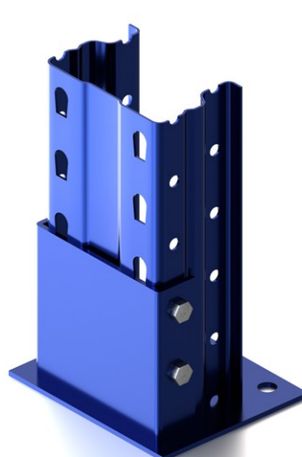
Upright 100 63 with base plate
