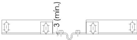
Plan view of 80 double corbel
