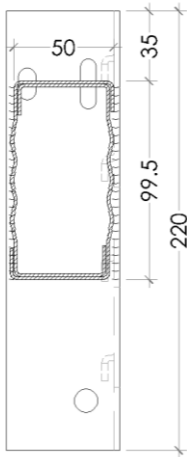
Cross-section A-A 100x50 beam
