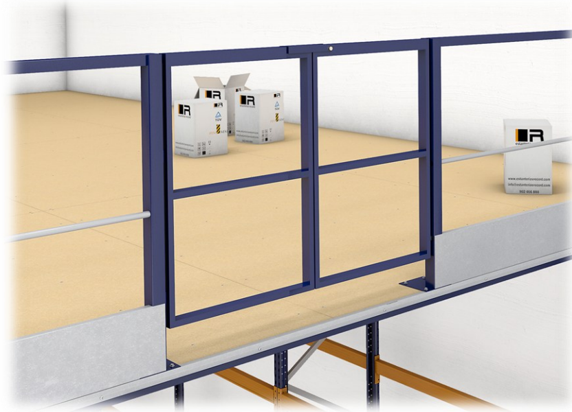
Hinged door in loft guardrail
