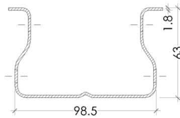
Plan view Upright 100 63
