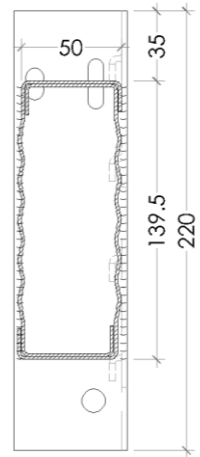
Cross-section A-A 140x50 beam
