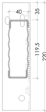
Cross-section A-A 120x40 beam
