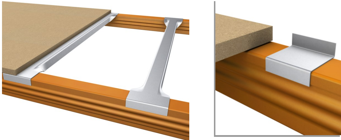
Conventional picking level with supports and retainer
